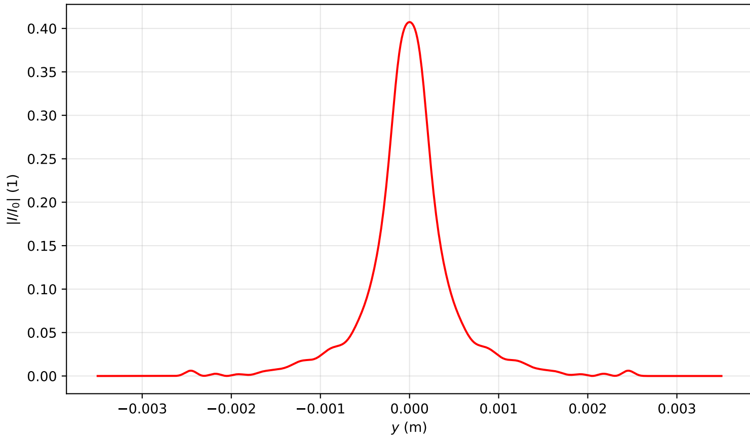
Intensity profile I(x=0, y, z=2.070)/I_0 , \text{Pin}=3.0\text{Pcr} , artificial time
